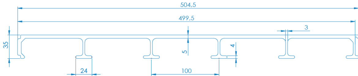
Figur 5: Geometrie Planke 500.35
